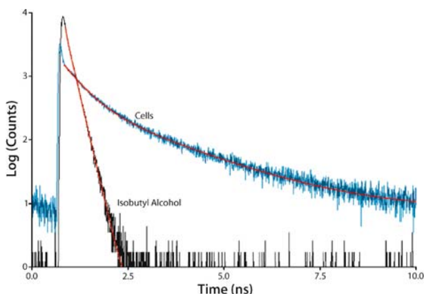
Fig. 8 Time-resolved fluorescence decay measurements establish the fluorescence lifetime. The cellular \text{ASP}^+ fluorescence lifetime was quantified using time-resolved fluorescence spectroscopy. The \text{ASP}^+ lifetime in the calibration solvent, isobutyl alcohol, and cellular lifetime was measured in a lifetime spectrometer. Cellular lifetime was measured by preloading hNET-293 cells with 5 \mu\text{M} \text{ASP}^+ for 10 min prior to harvest and washing. The log value for the photon counts is plotted against time, and the data are fit to the multi-exponential function ( \text{Counts} = A + Be^{-t/\tau} + Ce^{-t/\tau} + De^{-t/\tau} \dots )
