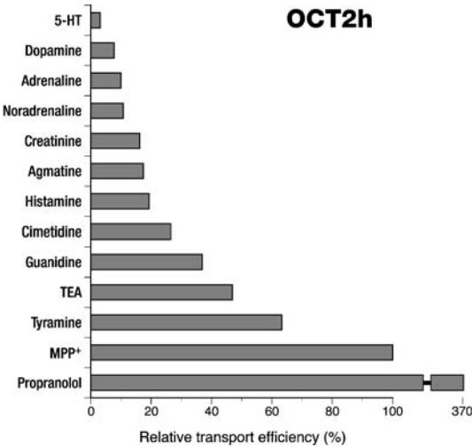
Fig. 3 Consensus TEs for OCT2h
