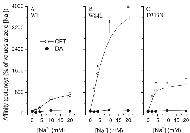
Fig. 1 A–C CFT affinity and DA inhibitory potency as a function of Na^+ concentration. A Wildtype (WT); B W84L; C D313N. Cell membranes were incubated with 4 nM [ ^3H ]CFT for 15 min at 21 °C in HEPES-Tris buffer containing various concentrations of Na^+ -ISE. Results are shown as the percentage of the binding affinity ( 1/K_D ) or inhibitory potency ( 1/K_i ) at zero [Na^+] . The K_D values for CFT at 0 and 20 mM [Na^+] were 95.3 and 11.6 nM at WT, 74.5 and 2.22 nM at W84L, and 38.8 and 2.45 nM at D313. The K_i values for DA at 0 and 20 mM [Na^+] were 7.3 and 6.27 \mu M at WT, 7.0 and 5.04 \mu M at W84L, and 6.3 and 4.25 \mu M at D313. Values represent means \pm SEM (standard error of mean) of 6 or more experiments performed in triplicate. * p < 0.05 versus the corresponding value for WT group (Dunnett's test). (Reprinted with permission from Chen et al. 2002, Fig. 4 therein)
