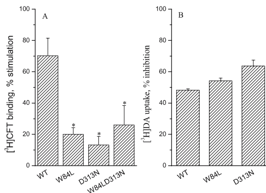
Fig. 3 A,B Relative response of [^3\text{H}]\text{CFT} binding and [^3\text{H}]\text{DA} uptake to \text{Zn}^{2+} upon mutation of W84 and D313. A [^3\text{H}]\text{CFT} binding. Cells were incubated with 4 nM [^3\text{H}]\text{CFT} and 10 \mu\text{M} \text{Zn}^{2+} in a \text{Na}^+ -free and NMDG-Cl substituted buffer for 15 min. Data are expressed as percentage stimulation of the binding in the absence of \text{Zn}^{2+} . B [^3\text{H}]\text{DA} uptake. Cells were incubated with 10 nM [^3\text{H}]\text{DA} and 10 \mu\text{M} \text{Zn}^{2+} in regular \text{Na}^+ -containing buffer for 5 min. Data are expressed as percentage inhibition of the uptake in the absence of \text{Zn}^{2+} . Shown are means \pm SE of three experiments performed in triplicate. * p < 0.05 versus the value at WT (Dunnett's test). (Reprinted with permission from Chen et al. 2004b, Fig. 8 therein)
