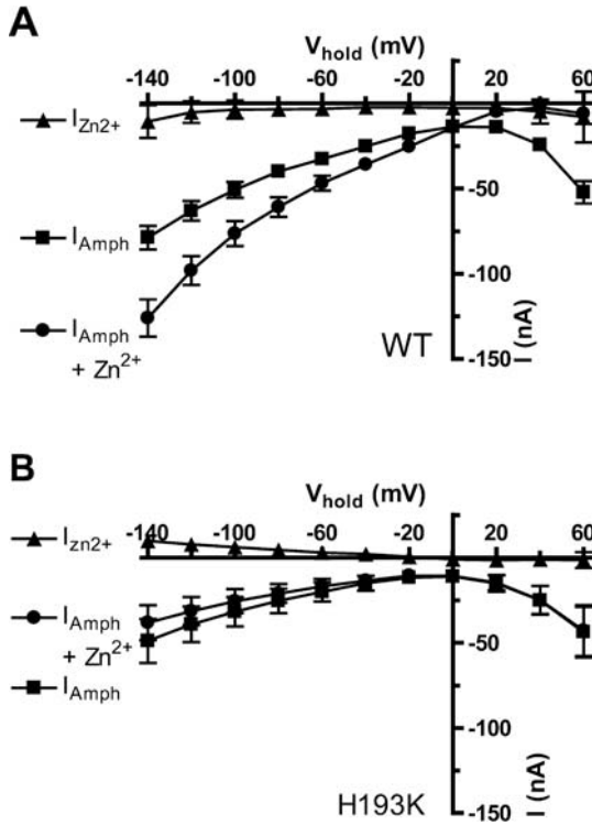
Fig. 2 A,B \text{Zn}^{2+} and substrate-mediated currents in Xenopus laevis oocytes expressing DAT wildtype (WT) or DAT H193 3,87 K (H193K). Current-to-voltage relationship of steady-state currents induced by either 10 \mu\text{M} amphetamine ( I_{\text{Amph}} ), 10 \mu\text{M} \text{Zn}^{2+} ( I_{\text{Zn}^{2+}} ), or 10 \mu\text{M} amphetamine (AMPH) plus 10 \mu\text{M} \text{Zn}^{2+} ( I_{\text{Amph}+\text{Zn}^{2+}} ). A Voltage dependence of the substrate-mediated currents in oocytes expressing hDAT WT (WT) ( n = 10 ). B Voltage dependence of the substrate-mediated currents in oocytes expressing the control mutant hDAT H193 3,87 K (H193K), which does not bind \text{Zn}^{2+} ( n = 5 ). Reproduced from Meinild et al. (2004)
