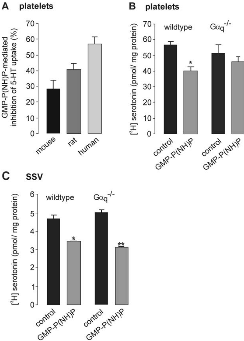
Fig. 3 A–C G\alpha_q regulates VMAT activity in platelets. A Platelets obtained from mouse, rat or human were permeabilized with SLO, and serotonin uptake was performed in the absence or presence of 50 \mu M GMP-P(NH)P as given (Höltje et al. 2003). Values (mean of three samples) were corrected for unspecific binding obtained in the presence of reserpine and are expressed as GMP-P(NH)P-mediated inhibition (%). B Platelets obtained from wildtype or G\alpha_q^{-/-} mice were subjected to serotonin uptake in the absence or presence of GMP-P(NH)P. From Höltje et al. (2003), with permission. C Synaptic vesicle obtained from wildtype or G\alpha_q^{-/-} mice (Höltje et al. 2003) were subjected to serotonin uptake in the absence or presence of 50 \mu M GMP-P(NH)P. Values (mean of three samples) were corrected for unspecific binding obtained in the presence of reserpine. Note that G\alpha_q regulates VMAT2 activity in platelets but not in brain
