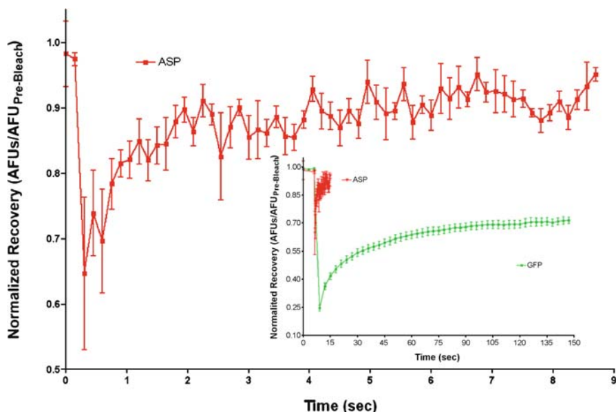
Fig. 11 FRAP experimentation cannot measure \text{ASP}^+ association rates. hNET-293 cells are exposed to 2\ \mu\text{M} \text{ASP}^+ . Several pre-bleach images were acquired prior to high-intensity light exposure. Several images were acquired, and \text{ASP}^+ recovered within 1 s. The inset shows the GFP-hNET and \text{ASP}^+ recoveries
