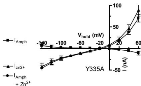
Fig. 4 Zn 2+ and substrate-mediated currents in Xenopus laevis oocytes expressing DAT Y335 6,68 A (Y335A). Current-to-voltage relationship of steady-state currents induced by either 10 \mu M amphetamine ( I_{\text{Amph}} ), 10 \mu M Zn 2+ ( I_{\text{Zn}^{2+}} ) or 10 \mu M AMPH plus 10 \mu M Zn 2+ ( I_{\text{Amph}+\text{Zn}^{2+}} ). Voltage dependence of the substrate-mediated currents in oocytes expressing the hDAT Y335 6,68 A mutant (Y335A) ( n = 8 ). Reproduced from Meinild et al. (2004)
