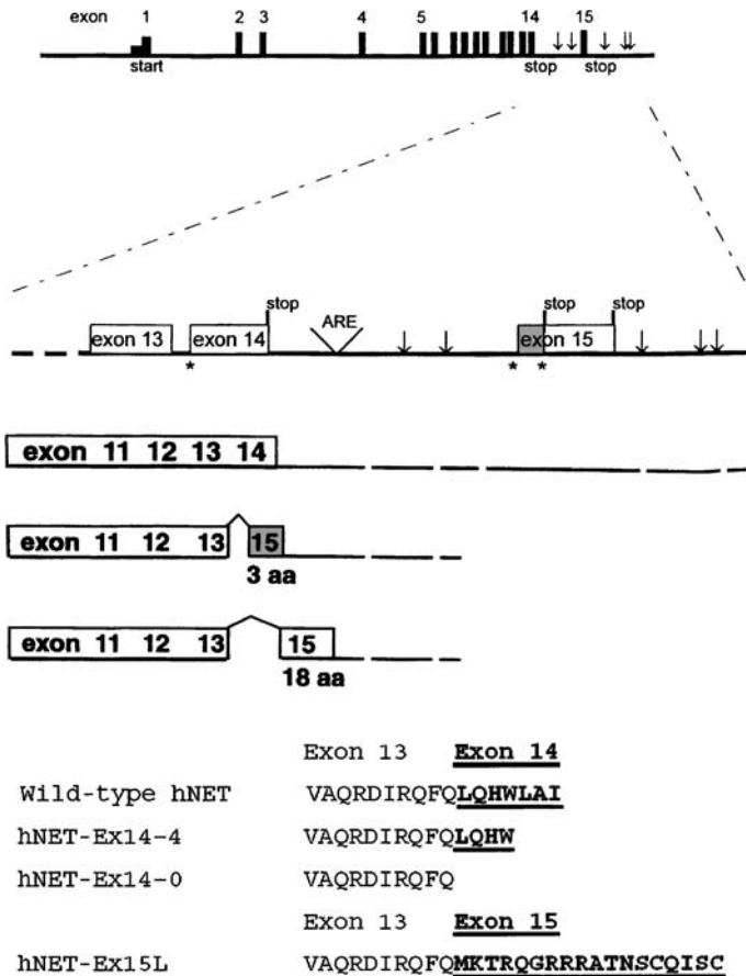
Fig. 2 Schematic representation of the hNET gene organization and of alternative splicing in the 3' region of hNET transcripts. Upper part of Fig. 2, hNET gene structure and alternative splicing; black vertical bars , exons 1–15; start , translational start codon; stop , translational stop codon; ARE , adenylate-rich region; arrows , polyadenylation signals; aa , amino acid. Lower part of Fig. 2, deduced C-terminal amino acid sequences of wild-type hNET and two artificial ( Ex14-4 and Ex14-0 ) C-terminal hNET variants as well as the long ( Ex15L ) hNET splice variant (see Distelmaier et al. 2004 for further information)
