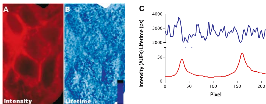
Fig. 7 A,B Frequency domain lifetime measurements. hNET-293 cells are exposed to 2\ \mu\text{M} ASP + for 5 min prior to image acquisition. The changes in fluorescence intensity (A) and fluorescence lifetime (B) were examined using fluorescence lifetime imaging microscopy (FLIM) (see Sect. 1.2). The color gradient in panel b indicates the fluorescence lifetime value with black as the longest lifetime. Using the identical imaging settings, increasing concentrations of ASP + in isobutyl alcohol and GFP in water were imaged ( right panel ). The average pixel intensity across an image plan 10\ \mu\text{m} from the coverslip was plotted against concentration [average \pm standard error of mean (SEM), n = 3 ASP + slope = 26.5\ \text{AFU}/\mu\text{M} , GFP slope = 15.3 \pm 0.41\ \text{AFU}/\mu\text{M} ]. C Line scan
