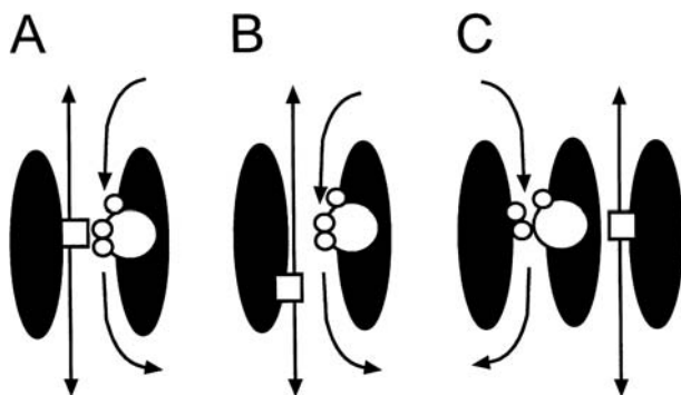
Fig. 6 A–C Three schematic models for the dual functions of glutamate transporters. A A single pore model where glutamate/ \text{Na}^+/\text{H}^+/\text{K}^+ binding to the transporter forms the \text{Cl}^- ion binding site. B A single pore model with separate molecular determinants for glutamate/ \text{Na}^+/\text{H}^+/\text{K}^+ and \text{Cl}^- . C A dual pore model with separate pores for glutamate/ \text{Na}^+/\text{H}^+/\text{K}^+ transport and the \text{Cl}^- channel. Key: large circle is glutamate, small circles are \text{Na}^+ ions, square is \text{Cl}^- ; \text{K}^+ and \text{H}^+ ions have been omitted
