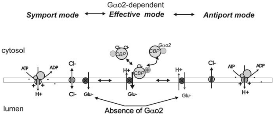
Fig. 7 Model describing the regulation of VGLUT activity by Gαo2. For details see text
