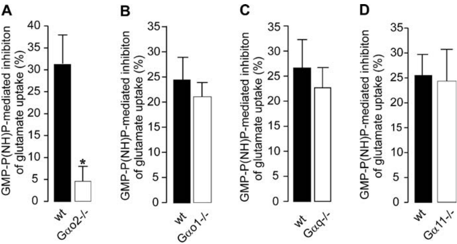
Fig. 5 Gαo2 regulates VGLUT activity. Glutamate uptake was performed into synaptic vesicles in the absence or presence of GMP-P(NH)P obtained from either wildtype ( wt ) or from the indicated G protein deletion mutants: Gαo2 A, Gαo1 B, Gαq C or Gα11 D. Values are the mean of two or three individual experiments and expressed as GMP-P(NH)P-mediated inhibition. From Winter et al. (2005), with permission
