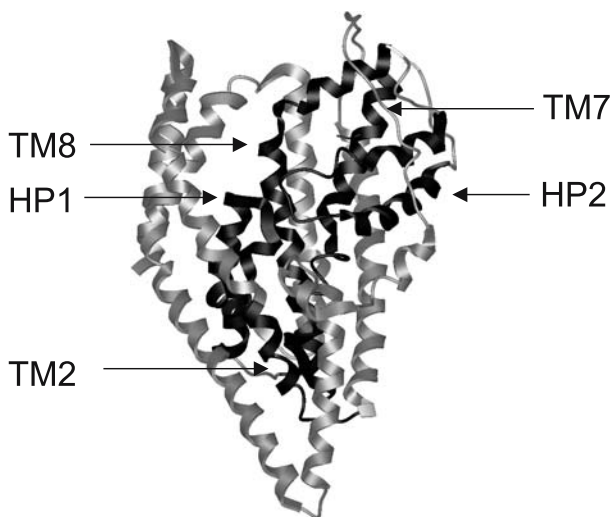
Fig. 7 Proposed transport and channel domains of glutamate transporters. HP1 and HP2 may form the internal and external gates of the transporter with TM7 and TM8 forming the glutamate/ \text{Na}^+/\text{H}^+/\text{K}^+ binding sites. TM2 may form part of the \text{Cl}^- channel. See text for details on the suggested movements of the various regions responsible for transport and channel activation
