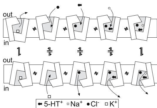
Fig. 1 Possible mechanism of serotonin transport. Transport of 5-HT together with Na + and Cl - ions requires binding of each solute to the transporter. These binding events are depicted in the three steps on the upper right of the figure. There is no evidence that the binding sequence is strictly ordered. Only after all three solutes are bound is the transporter able to undergo a series of conformational changes that closes off access to the extracellular medium and exposes the binding site to the cytoplasm. This conformational change is depicted on the right side of the figure. After dissociation of 5-HT, Na + , and Cl - on the cytoplasmic side of the plasma membrane, as shown by the three rightmost steps on the lower part of the figure, a cytoplasmic K + ion is able to bind ( lower left ). Once K + has bound, SERT is able to undergo another series of conformational changes that closes off access to the cytoplasm and exposes the binding site to the extracellular medium. Dissociation of K + to the medium completes the cycle. Note that for effective coupling of 5-HT influx to both influx of Na + and Cl - and efflux of K + , transitions between the extracellular-facing and cytoplasmic-facing forms of SERT should occur only when the binding site is occupied with 5-HT, Na + , and Cl - or with K +
