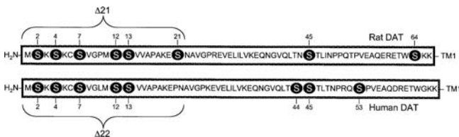
Fig. 3 Schematic depiction of DAT N-terminal tail phosphorylation sites. The N-terminal amino acid sequences of rat ( upper ) and human ( lower ) DATs through transmembrane domain 1 (TM1) are depicted with potential serine phosphorylation sites highlighted with black circles and white letters . Mutants with the deletion of 21 N-terminal amino acids in rat DAT ( \Delta 21 ) and 22 N-terminal amino acids in human DAT ( \Delta 22 ) are indicated by the brackets
