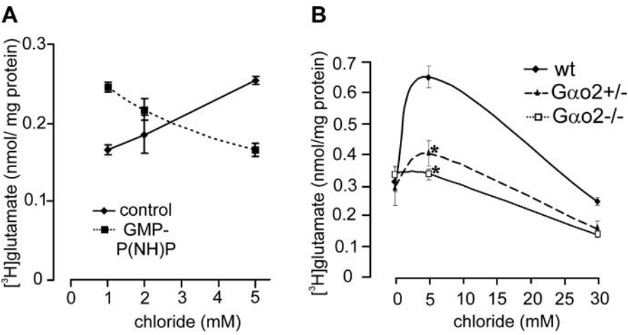
Fig. 6 A,B Gαo2 regulates the chloride dependence, of VGLUT. A Glutamate uptake was performed in synaptic vesicles in the absence or presence of GMP-P(NH)P using the chloride concentrations given at the abscissa . B Chloride dependence of VGLUT activity is reduced or diminished into SSV from heterozygous or knock-out animals, respectively. From Winter et al. (2005), with permission
