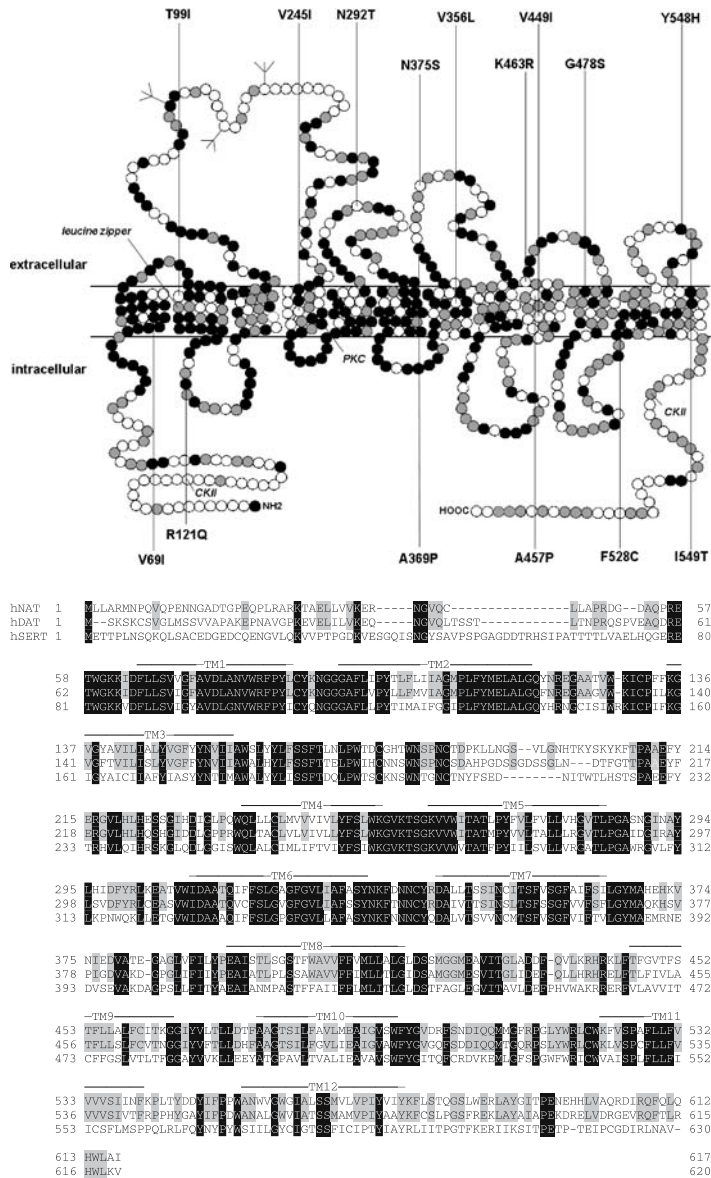
Fig. 1 Proposed topology of the human NET depicting 12 transmembrane domains (TMs) (upper part), and alignment of the human NET with the human DAT and human SERT (lower part). The upper part also indicates naturally occurring hNET variants, a leucine zipper in TM2, N-glycosylation sites within the second extracellular loop and intracellular residues which are potential sites for phosphorylation by protein kinase C (PKC) or casein kinase II (CKII). Amino acids conserved between hNET and hDAT are indicated in both parts in grey and those conserved between all three transporters in black
