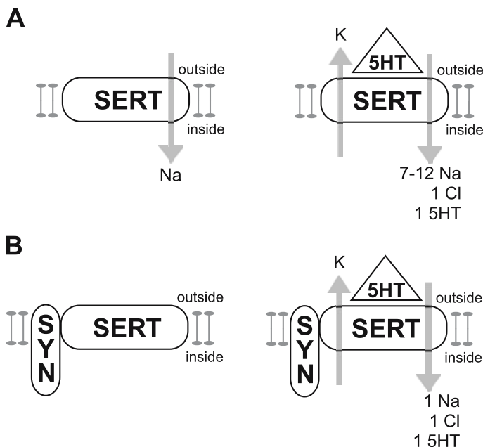
Fig. 2 A,B Syntaxin 1A regulates conducting states of SERT. A In the absence of serotonin, SERT shows \text{Na}^+ leak currents. In the presence of serotonin (5HT), substrate translocation is electrogenic. The current is carried by a variable, voltage-dependent flux of \text{Na}^+ ions. B In the presence of syntaxin 1A (SYN), the \text{Na}^+ leak conductance is eliminated, and transport is electroneutral
